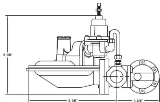
1883CPB2 Regulator
