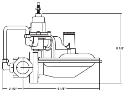
1800CPB2 Regulator
