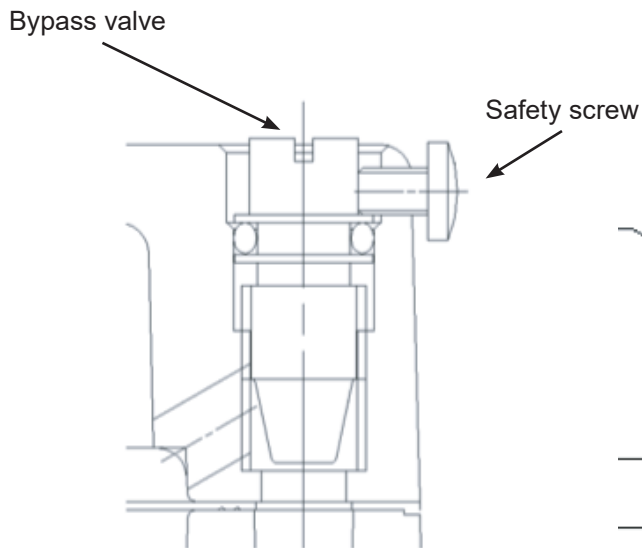
Figure 3 Bypass valve adjustment on BR200 model
