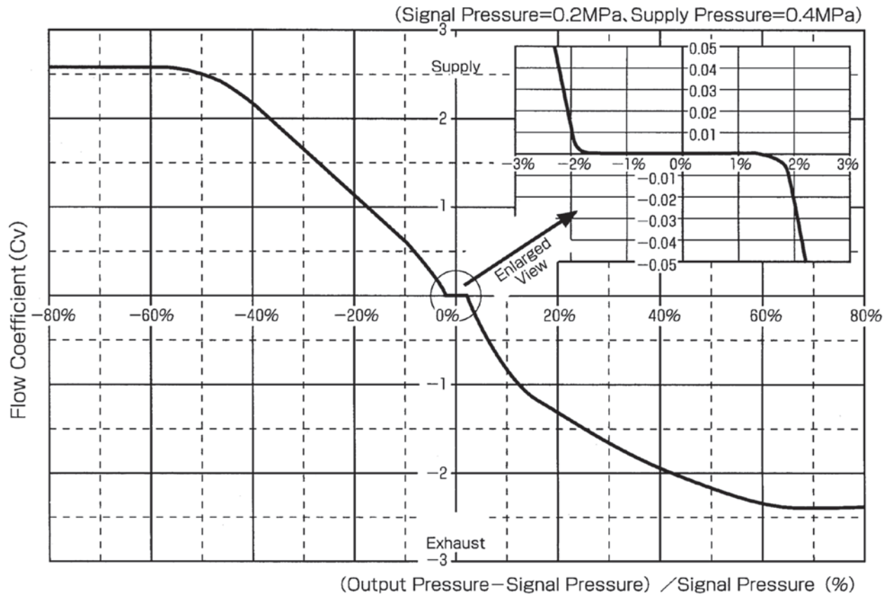
Figure 2 - Flow Characteristics
