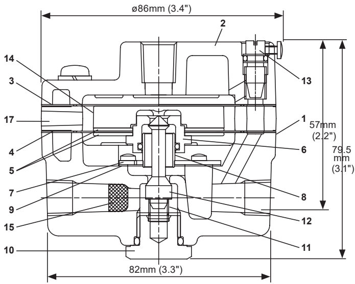
Figure 5 - BR200 Construction and Dimensions
