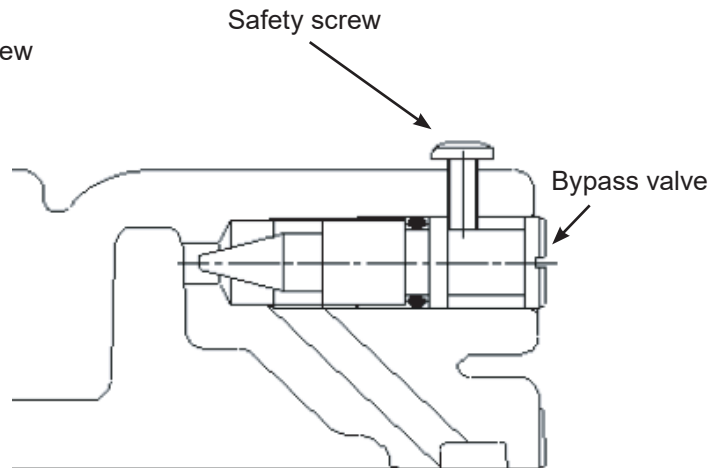
Figure 4 Bypass valve adjustment on BR400 model
