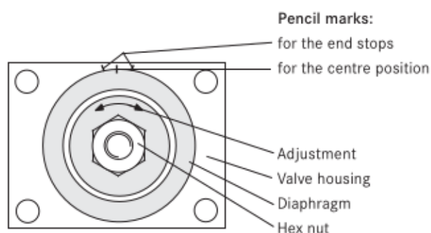
Fig. 2: Diaphragm system
