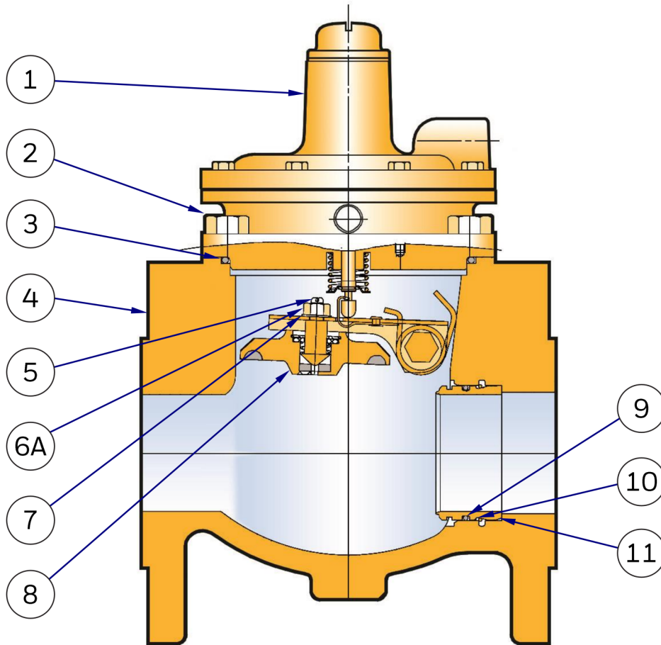
SLAM SHUT ASSEMBLY Fig. 5
