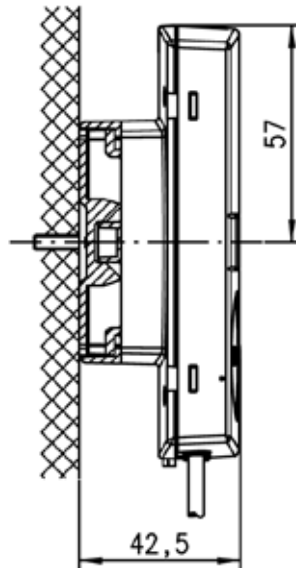
Fig. 18: Wall mounting
