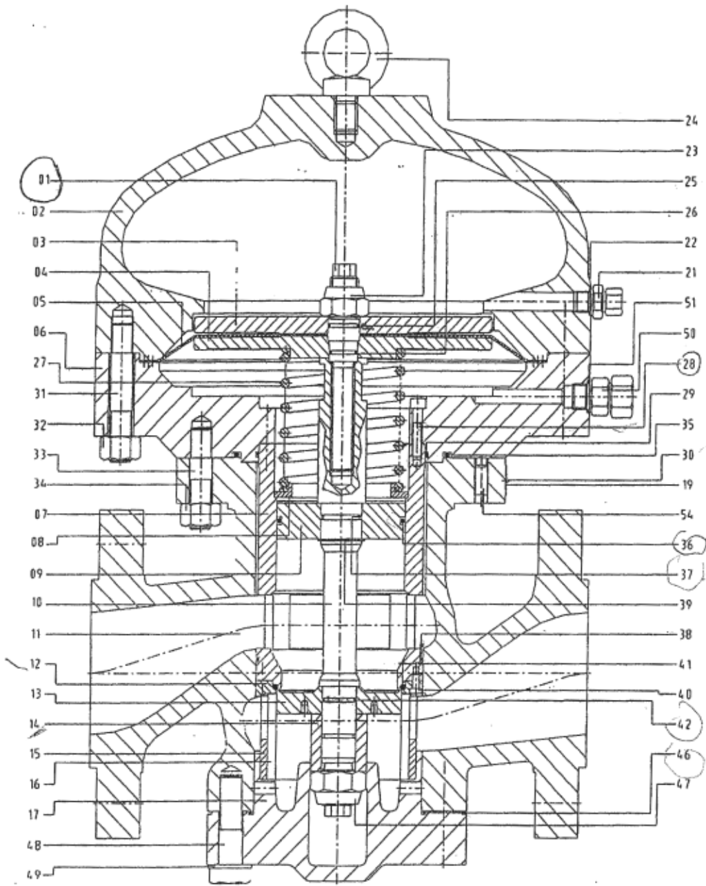
Figure 5.3: Component drawing R100(S)-2" to 8"
