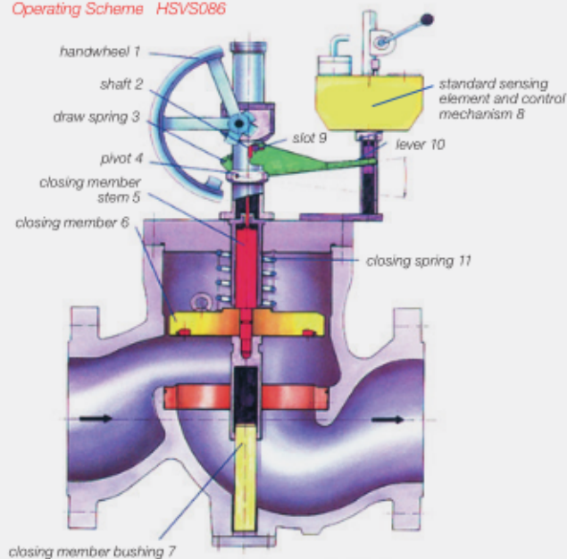
Operating Scheme HSVS086
