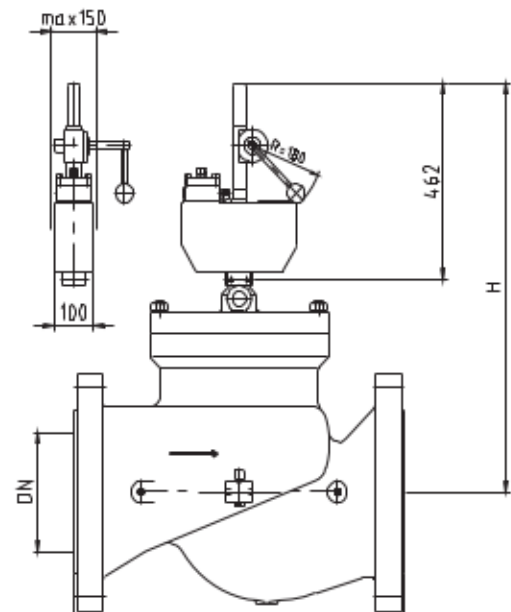
Dimensional sketch HSV086
