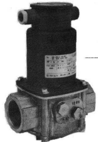
Type GS Solenoid Valves Fast Opening 1/2"2 BSPP
