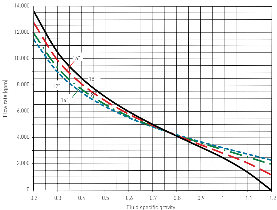
FIGURE 3 12" to 18" pivot type ITV maximum allowable fill rates
