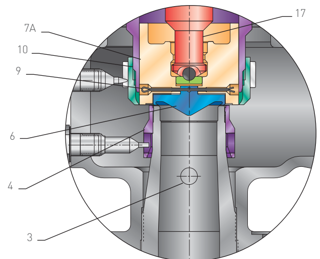
K - QQ ORIFICE CONSTRUCTION
