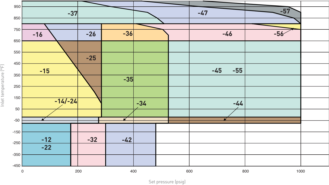
PRESSURE/TEMPERATURE LIMIT CHART P Orifice, 6.38 sq.in. (4116 sq.mm) API effective area
