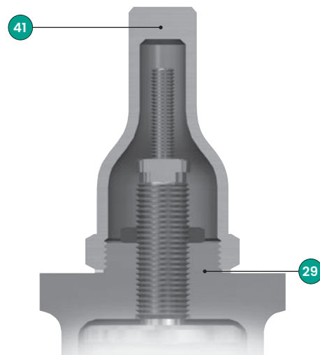
Screwed Cap Organic Fluid Vaporizer Application
