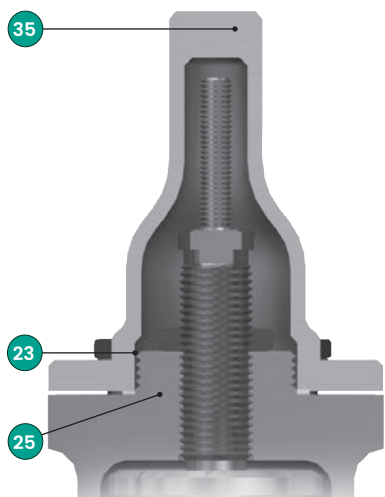
Bolted Cap Organic Fluid Vaporizer Application
