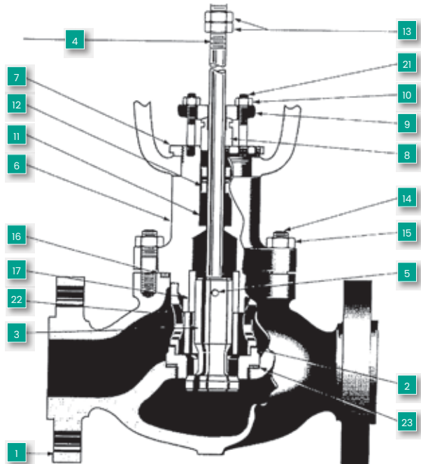
536 H Regulator Quick Change Trim Only (Detail)
