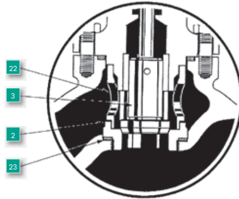
535 H Regulator Quick Change Trim (Detail)
