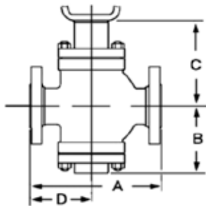
Flanged Ends
