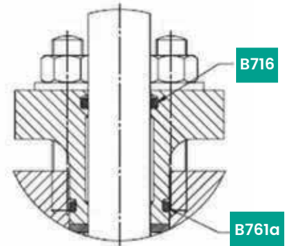
Packing Flange/Follower O-Ring Detail
