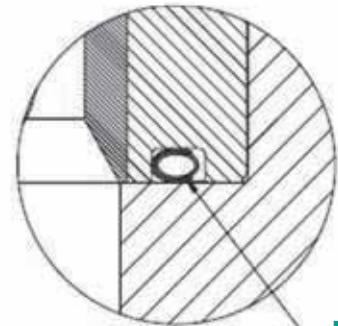
Flow-to-Close Seat-Ring Gasket Detail
