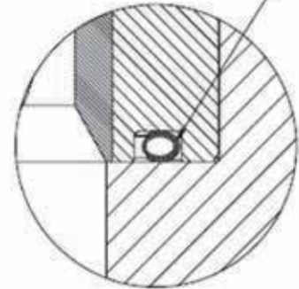
Flow-to-Open Seat-Ring Gasket Detail
