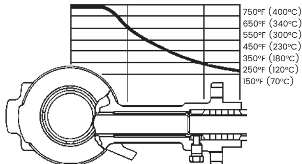
Temperature Gradient Across Standard Integral Bonnet
