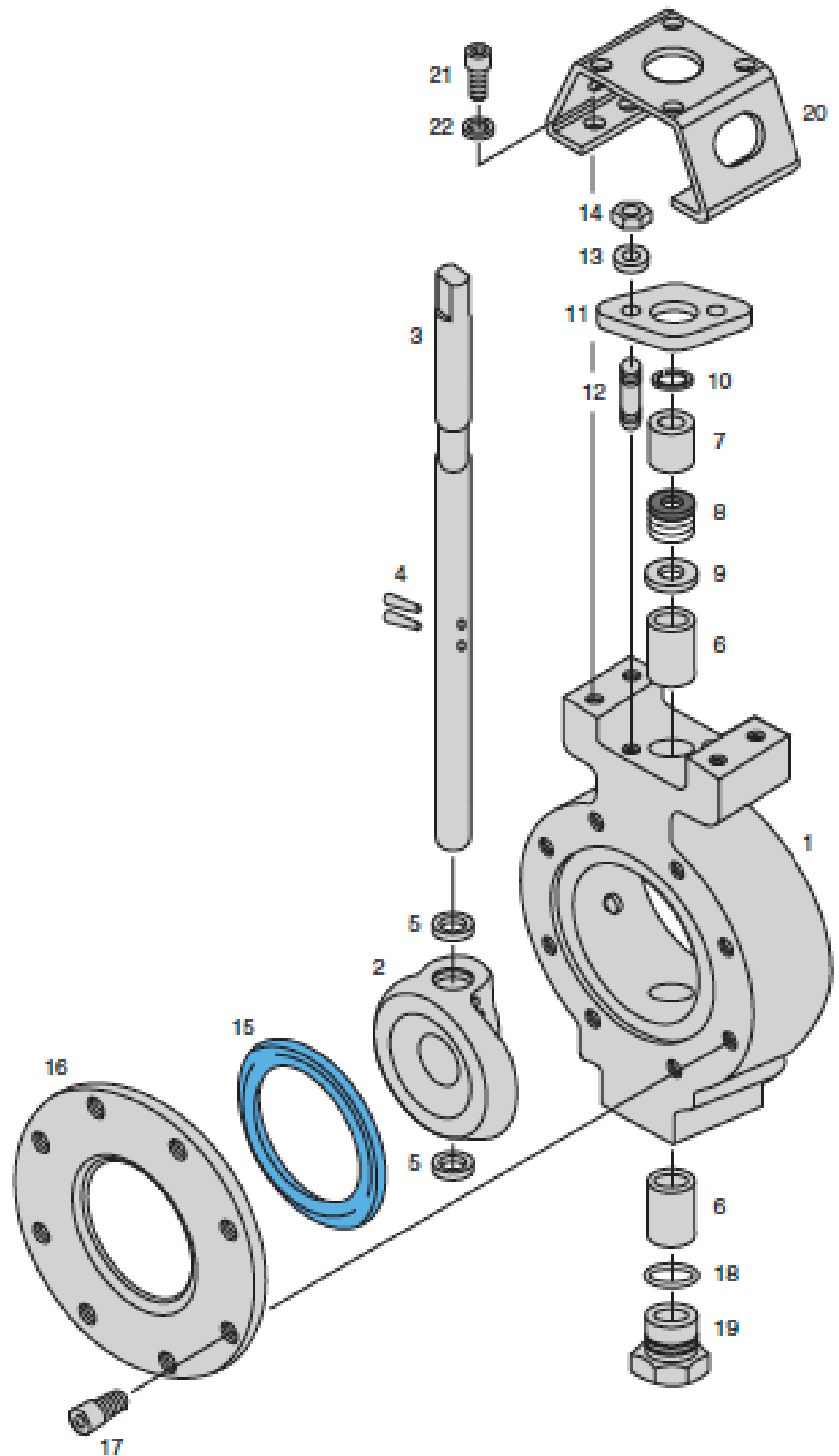
Exploded View
